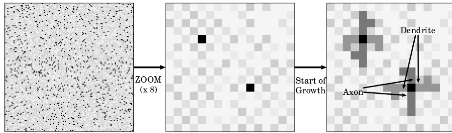
Fig. 6. (Left) An initial pattern of 128 \cdot 128 CA cells with a neuron-density of 5%. The (black) neuron cells are randomly positioned. (Middle) A zoom (x8) with two neuron cells on a random (2-cell gridded) chromosome. (Right) The beginning of the growth phase, after three CA-steps.
