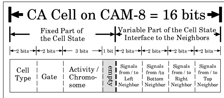
Fig. 4. State representation in the new CAM-Brain model, which uses 15 of the 16 bits in the CAM-8 CA-cell. During the growth phase 3 of the bits are used to store the chromosome’s growth instructions. The same 3 bits are later used to store the activity of a neuron cell during the signaling phase.
