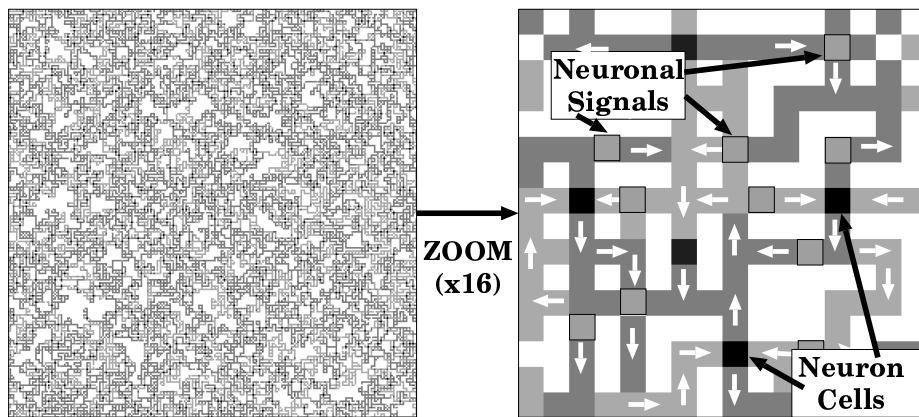
Fig. 5. (Left) A CA-space with 256 \cdot 256 cells in the signaling phase with the CoDi-model. (Right) A zoom (x16) with five neuron cells (black) with two dendrites and two axons each. The arrows inside the axonic (dark grey) signal trails and dendritic (light grey) signal trails indicate the direction of information flow during the signaling phase. In the growth phase the signals in the dendritic trails travel the other way, because they are emitted by the neuron. To improve the visualization of neural trails, the underlying chromosome is gridded with a checker-board pattern of “grow-straight” instructions. This causes the neural trails to grow on a 2-cell grid.
