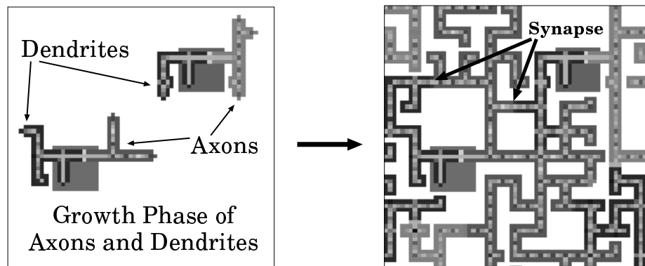
Fig. 3. (Left) The growth phase of the network continues until all CA trails are connected through synapses or are blocked. (Right) A network, fully grown with the old CAM-Brain model.
